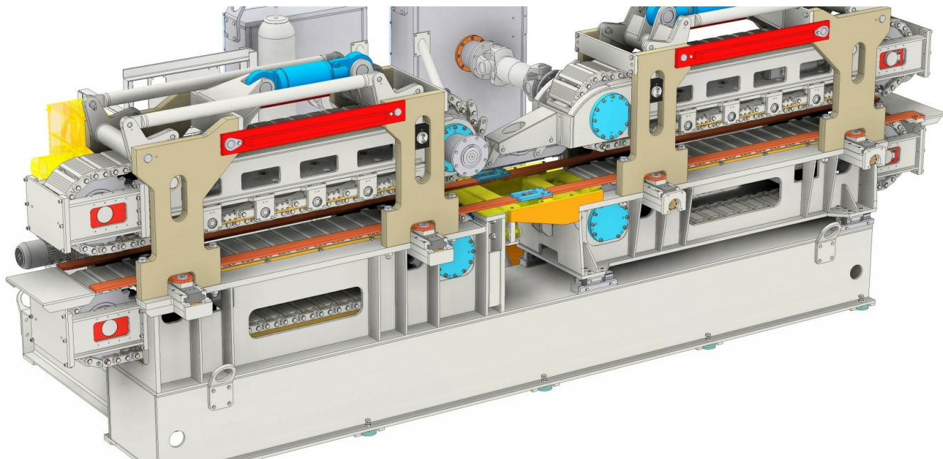
LEDINEK - FINGER JOINTING - KONTIZINK H 3000
